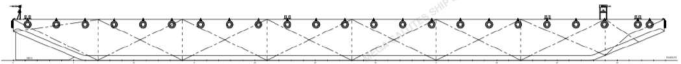
OUTBOARD PROFILE
